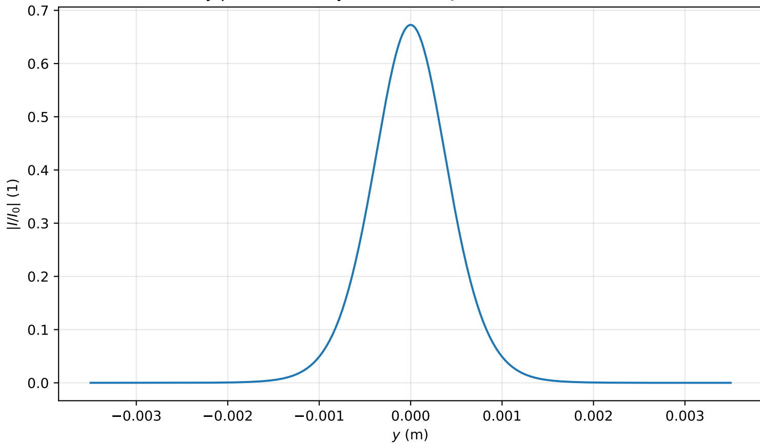
Intensity profile I(x = 0, y, z = 2.548)/I_0 , P_{in}=0.5P_{cr} , artificial time
